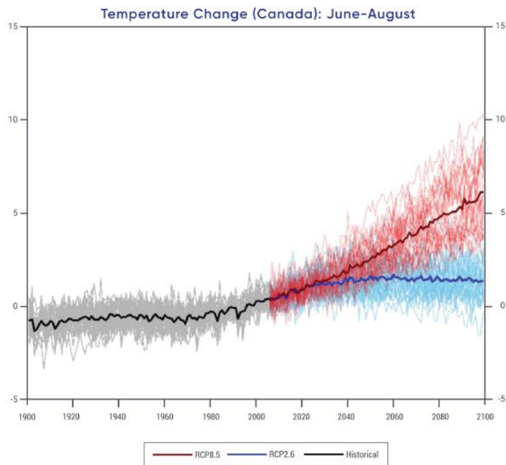
Figure 4.7: Projected temperature changes for summer season
