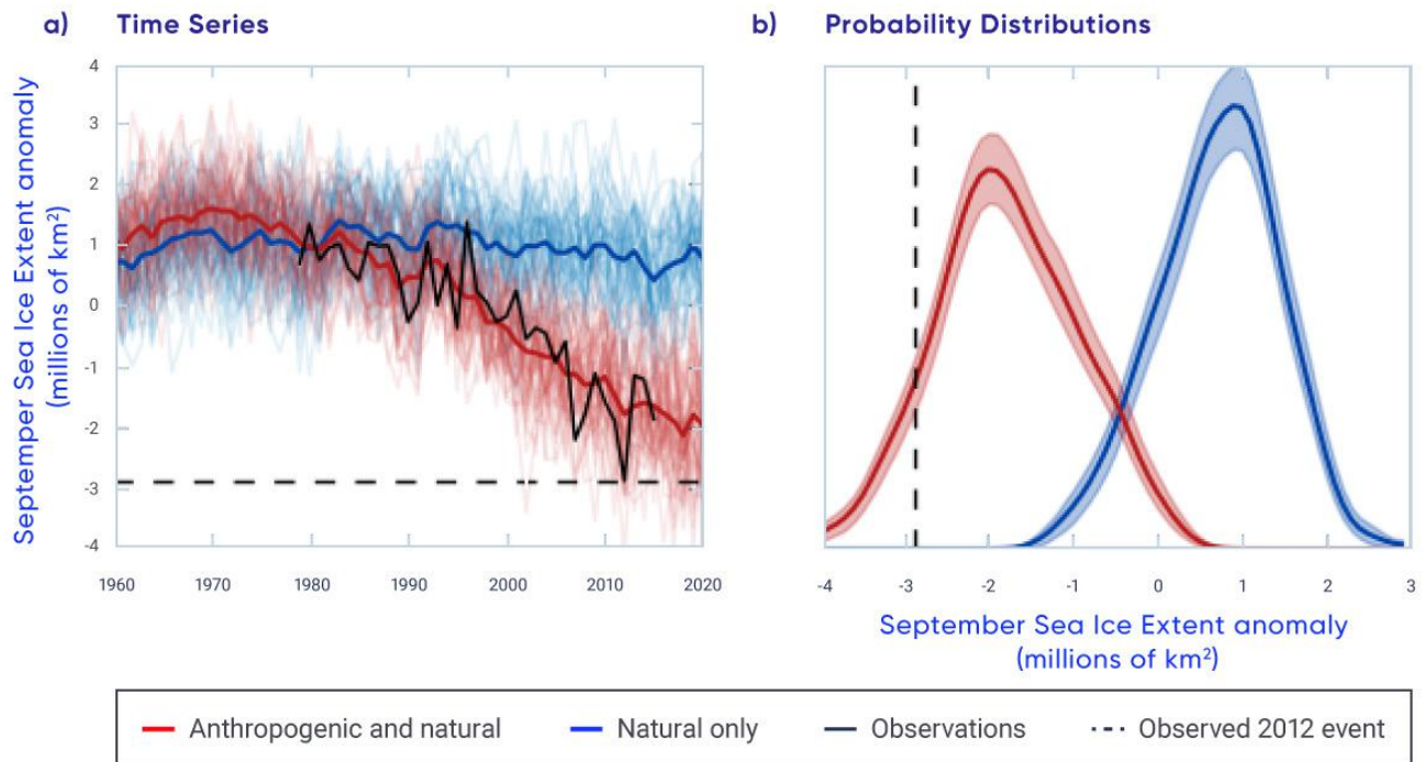
Figure 5.9: Comparison of Arctic sea ice extent between simulations with and without the contribution of human activities
