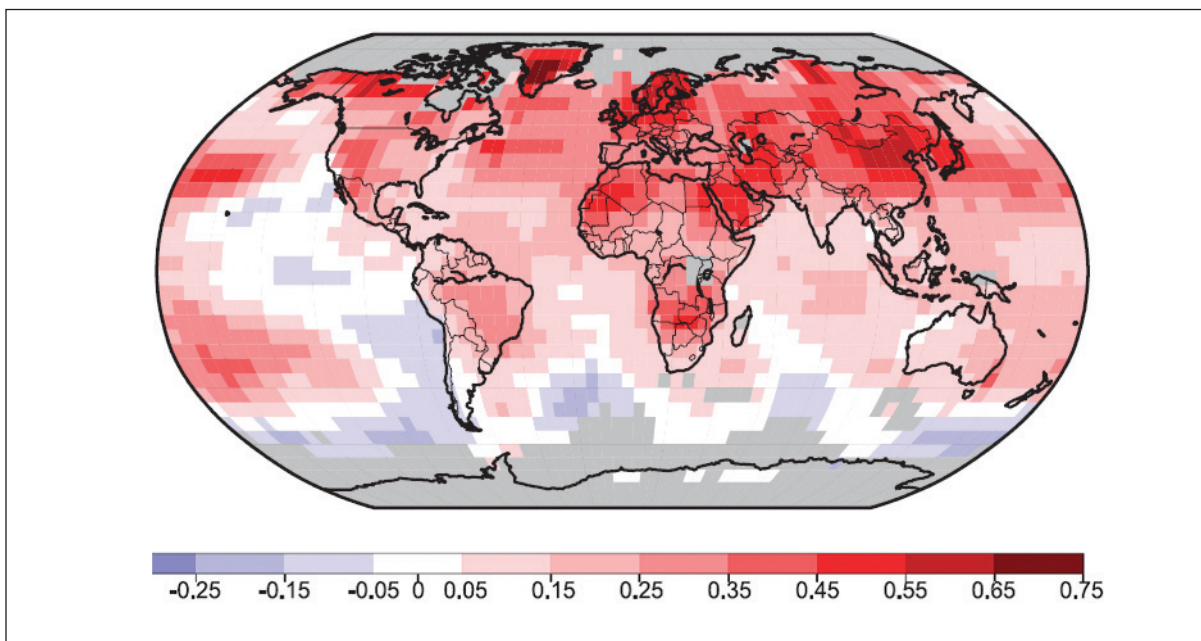
Figure 2. Patterns of linear global temperature trends from 1979 to 2005 estimated at the surface in °C per decade. Grey areas indicate incomplete data. 9
