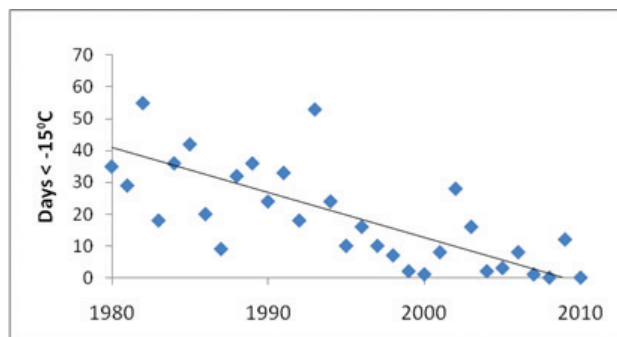
Figure 19. Winter days with temperatures below -15°C in Calgary.
