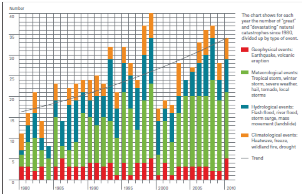
Figure 5. The number of "great" and "devastating" natural catastrophes (as defined by Munich Re) since 1980, indicated by type of event.
