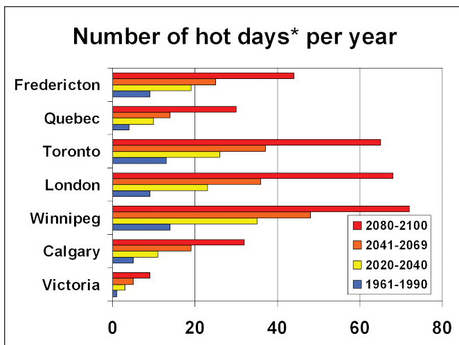
Figure 9. The number of hot days (days with a maximum temperature over 30°C) projected for several Canadian cities by Environment Canada.
