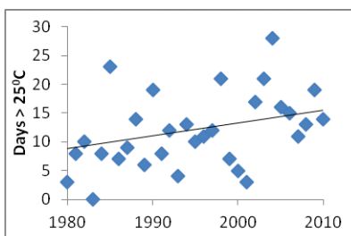
Figure 20. Observed trends of hot summer days in Vancouver.
