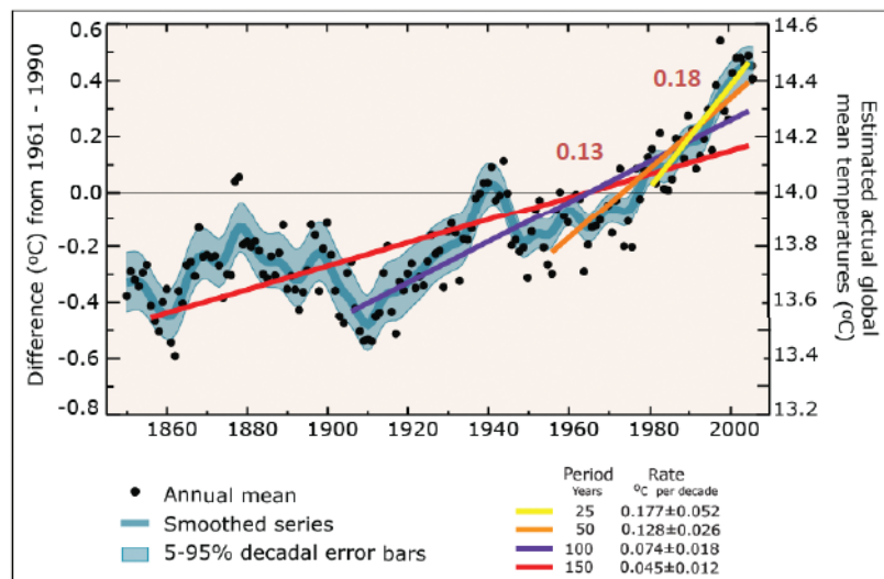
Figure 1. Annual global mean temperatures (black dots) with linear fits to the data. The left-hand axis shows temperature anomalies relative to the 1961 to 1990 average and the right-hand axis shows estimated actual temperatures, both in ^{\circ}\text{C} . Linear trends are shown for the last 25 (yellow), 50 (orange), 100 (magenta) and 150 (red) years. The smooth blue curve shows decadal variations with the decadal 90% error range shown as a pale blue band about that line. The total temperature increase from the period 1850 to 1899 to the period 2001 to 2005 is 0.76^{\circ}\text{C} \pm 0.19^{\circ}\text{C} . The numbers in red show the linear trends in ^{\circ}\text{C} per decade for the past 50 years (0.13) and last 25 years (0.18). 6
