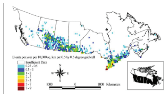
Figure 12. Observed tornado frequencies in Canada. 46
