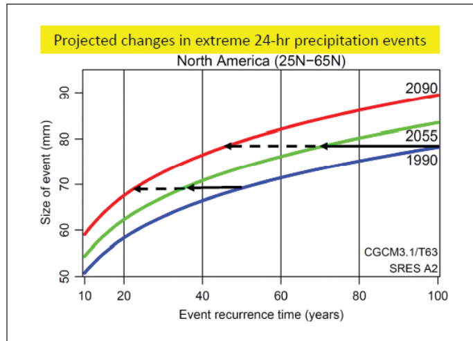
Figure 11. Projections of the event recurrence time (in years) for extreme precipitation events of a given magnitude (Environment Canada, based on the IPCC A2 scenario).
