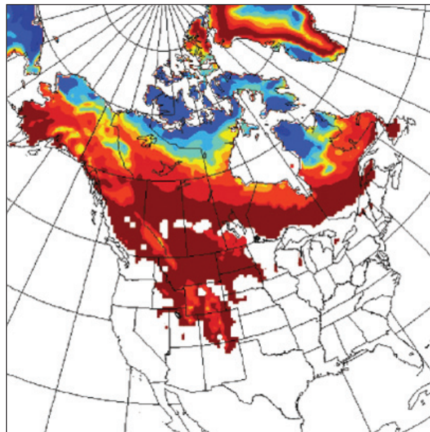
Figure 6. Percent changes in snow depth in March for mid-century (averaged over the period 2041 to 2070) under IPCC A2 emissions scenario, compared to the 1961 to 1990 period. The calculation is only done where climatological snow amounts exceed 5 mm of water equivalent. From IPCC. 35
