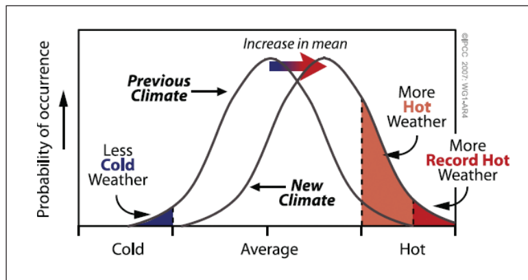
Figure 7. Schematic showing the effect on extreme temperatures when the mean temperature increases, for a normal temperature distribution. From IPCC. 38
