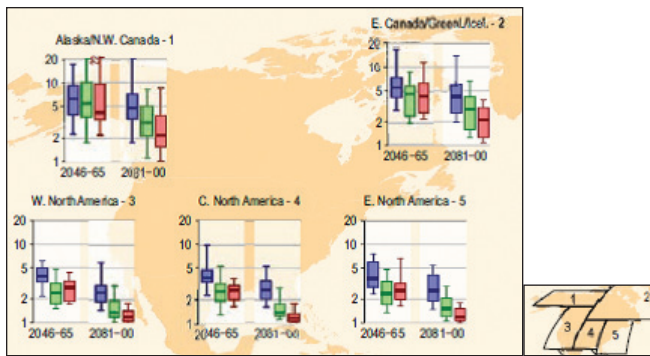
Figure 8. Projected return periods for the maximum daily temperature that was exceeded on average once during a 20-year period in the late 20th century (1981–2000). The box plots show results for regionally averaged projections for two time horizons, 2046 to 2065 and 2081 to 2100, compared to the late 20th century, and for three different emissions scenarios (from the IPCC’s Special Report on Emissions Scenarios, or SRES) (B1, blue; A1B, green; A2, red). The boundaries of the regions are shown in the lower right. From IPCC. 41
