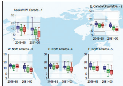
Figure 10. Projected return periods for a daily precipitation event that was exceeded in the late 20th century on average once during a 20-year period (1981–2000). The box plots show results for regionally averaged projections for two time horizons, 2046 to 2065 and 2081 to 2100, compared to the late 20th century, and for three different SRES emissions scenarios (B1, blue; A1B, green; A2, red). The boundaries of the regions are shown in the lower right of Figure 8. From IPCC. 42
