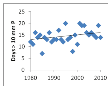
Figure 16. Trend of extreme precipitation days during winter in St. John's.
