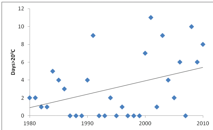
Figure 21. Trends in hot summer days in Iqaluit.
