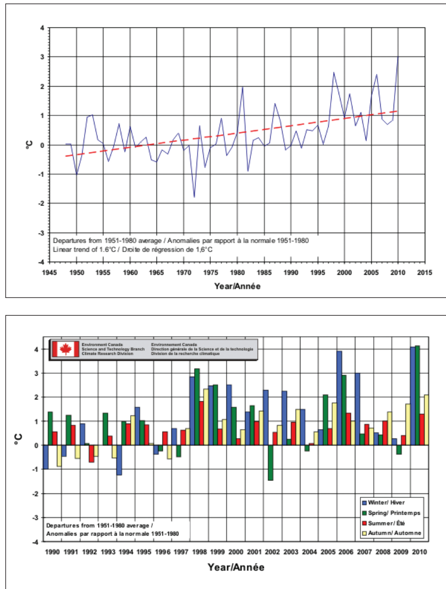
Figure 3. Annual temperatures averaged over Canada, as departures from 1951–1980 average, from 1948 to 2010 (top). Seasonal mean temperatures from 1990 to 2010 (bottom). 11
