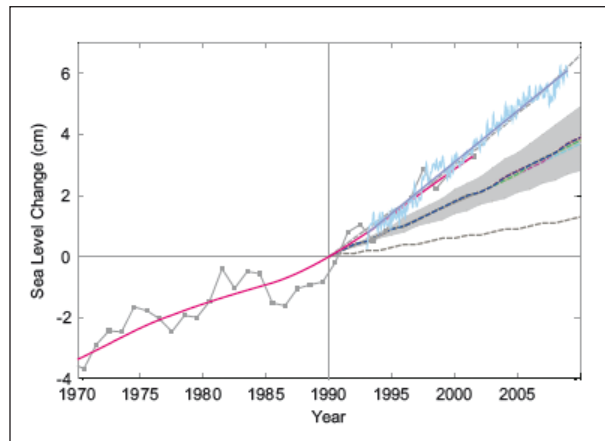
Figure 14. Change in sea level from 1970 to 2008, relative to the sea level at 1990. 56 The annual observations are shown by the dots connected by the light line. The light blue line from the mid-1990s to 2008 reflects new satellite observations. The solid red line represents the observations smoothed to remove the effects of interannual variability. The envelope of IPCC projections from 1990 is shown for comparison. The three short dash lines represent individual projections depending on the IPCC emissions scenario. The “most likely” scenario, based on analyses in 2000 is the middle scenario, which has shading around it to indicate the uncertainty. Note that the satellite observations follow along what was considered the upper limit of sea level rise for the period 2000–2010.
