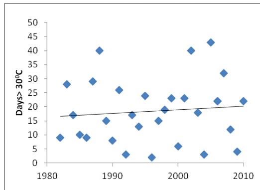
Figure 17. Number of days in the summer where the maximum temperature at Toronto Pearson Airport was above 30°C.
