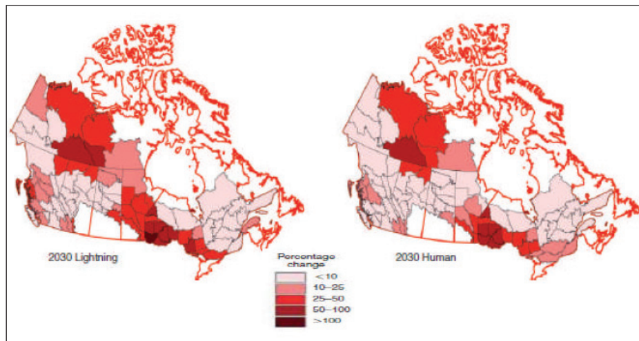
Figure 13. Relative change (% increase) in fire occurrence between future and baseline scenarios for the Canadian model due to lightning (left) and human activities (right). Relative change is given as the percentage increase in the number of fires predicted divided by the total number of fires in baseline. For the 2030 period, the largest percentage changes in the total number of fires are in Ontario and the Northwest Territories, both at 46%.
