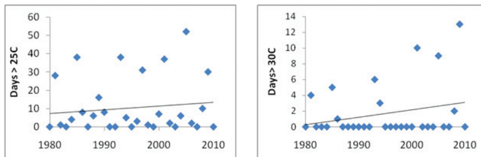
Figure 18. Summer days with temperatures above 25°C (left) and 30°C (right) in Calgary.
