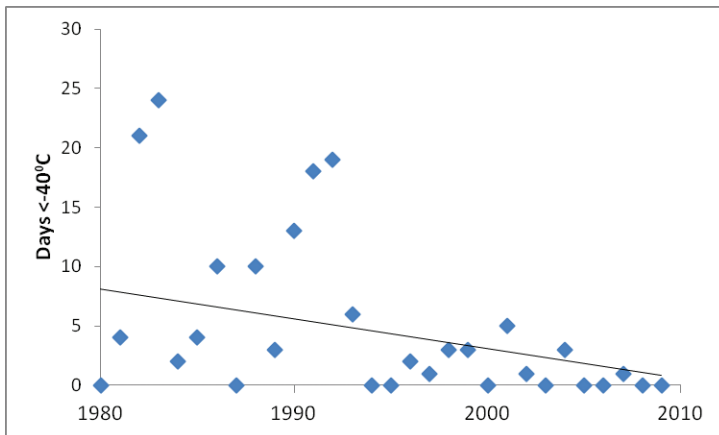
Figure 22. Trends in extreme cold on winter days in Iqaluit.
