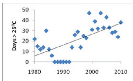
Figure 15. Trends of days with temperatures above 25°C during summer in Halifax, 1980–2010.
